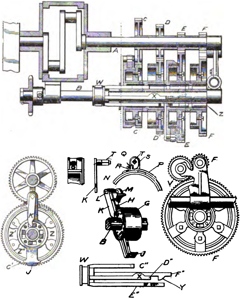
FIG. 334.—The Haynes-Apperson Change Speed and Reversing Gear. A is the first motion shaft; B, the secondary shaft; C, D, E and F, spur pinions keyed to A; C', D', E', F', pinions turning loose on B; G, drum keyed to B, on which the gears rotate loosely; H and J, arms cast integral with G; K, a lever arm pivoted at L on pin connected between bearings, M and N; P, forged nut of the strap around drum turning on G; Q, lug at end of P; R, an adjusting screw bearing against dog, S, carried on the same pivot as K; T, square portion of the pivot of K, to which is attached dog, S; V, an idler pinion giving reverse movement between A and B when gears F and F' are in gear. W is a spool for engaging a lever in sliding the sleeve, having the four fingers, C', D', E', F"; X and Y, lugs for clutching lever, K, on C', D', E' and F'; Z, channels in which the four fingers of the sleeve slide.
